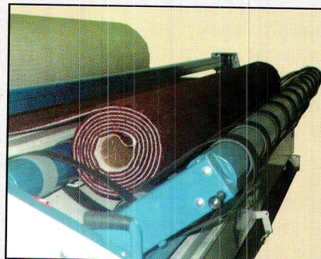
REVERSE ROLL
